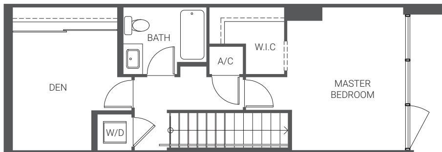
UPPER FLOOR
